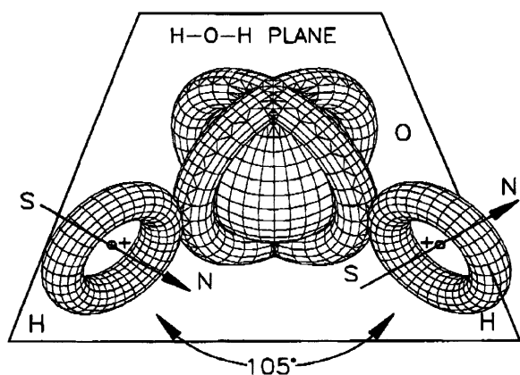
Fig. 17. A conceptual rendering of the conventional water molecule without any electric polarization. This rendering is primarily intended to illustrate the experimentally established feature that the orbitals of the two hydrogen atoms do not have a spherical distribution as in Fig. 13, but have instead a distribution essentially perpendicular to the H–O–H plane (see Ref. [1a,1b] for details) here conceptually represented with a toroid. The strong valence bond needed to achieve the first known exact representation of the experimental data of the water molecule achieved in Ref. [3] requires that the corresponding orbitals of the valence electrons of the oxygen have a corresponding polarized distribution here also conceptually depicted with toroids perpendicular to the H–O–H plane around the spherical core of the remaining electrons of the oxygen atom.
