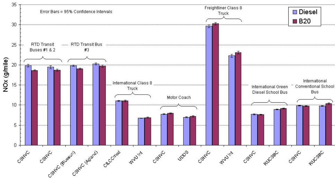
Figure 11. Comparison of NO x emissions for conventional diesel and B20 for each vehicle tested and each cycle.
